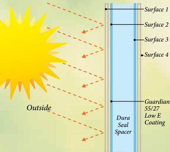
Eco-View with Low E Glass Guardian 55/27 Low E Coating is applied to the 2nd surface.
